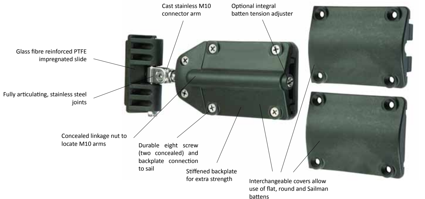
Series 55 U01520Y luff box, which includes 2 additional covers, shown
